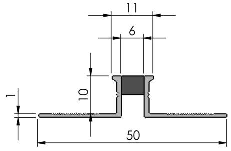
Section view
