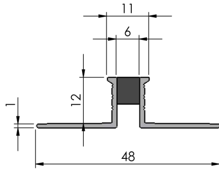
Section view
