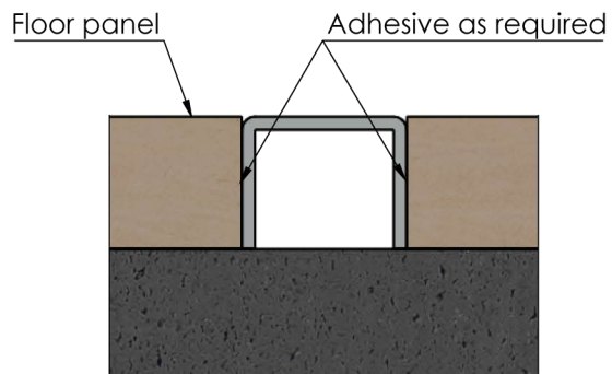
Typical installation detail
