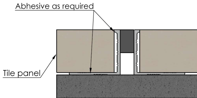
Typical installation detail
