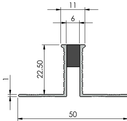
Section view
