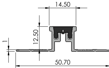
Section view
