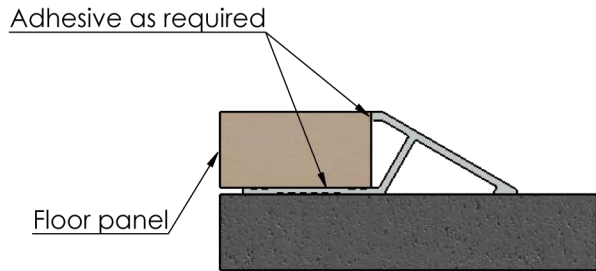
Typical installation detail
