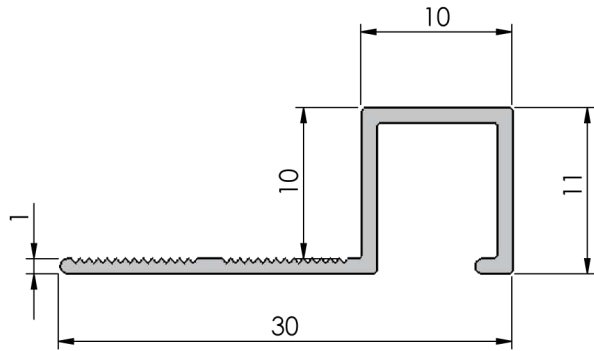
Section view
