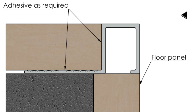
Typical installation detail
