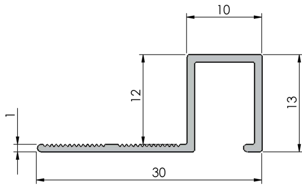
Section view
