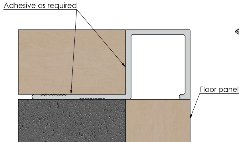
Typical installation detail
