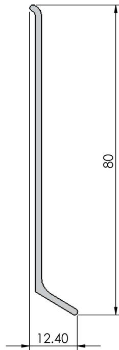
Section view
