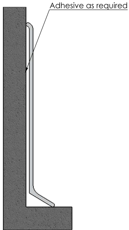
Typical installation detail
