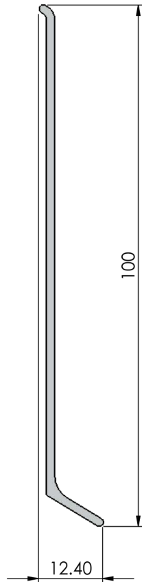
Section view
