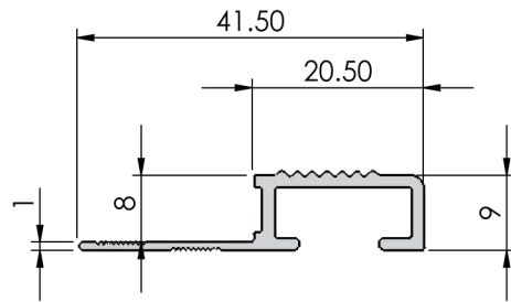
Section view
