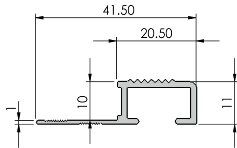
Section view
