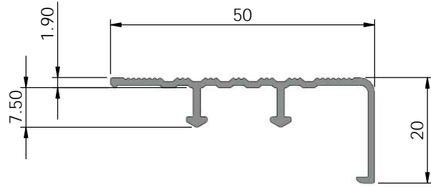
Section view
