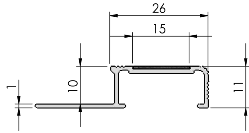
Section view
