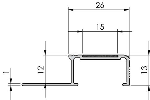
Section view
