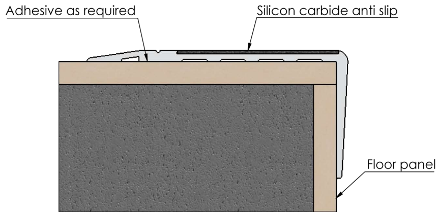
Typical installation detail
