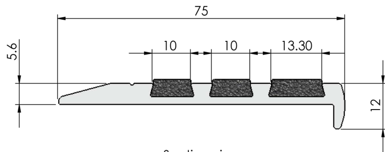
Section view
