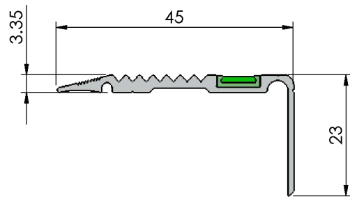
Section view
