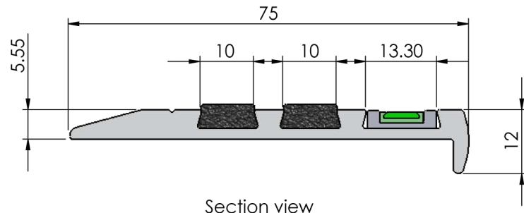
Section view
