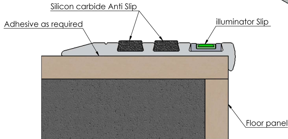
Typical installation detail
