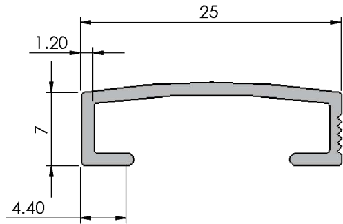
Section view
