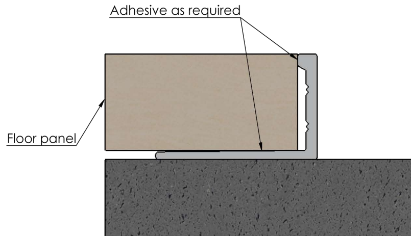
Typical installation detail
