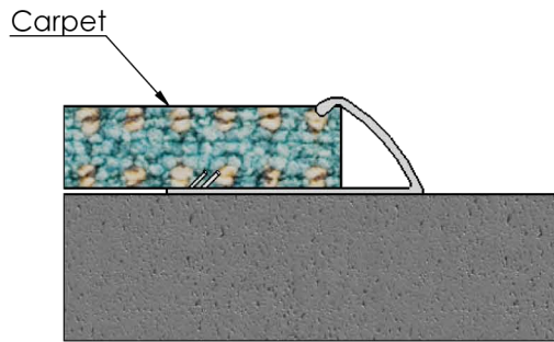
Typical installation detail
