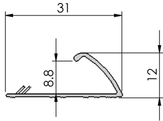
Section view
