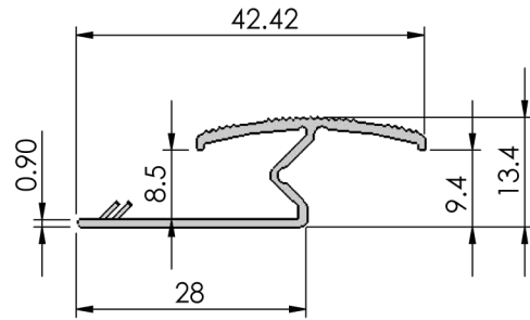
Section view
