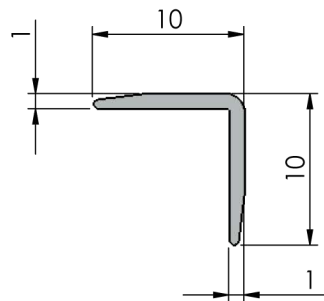
Section view
