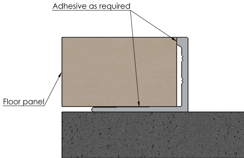
Typical installation detail
