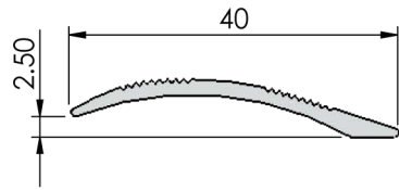
Section view
