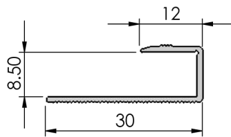
Section view
