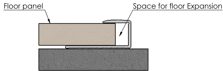
Typical installation detail
