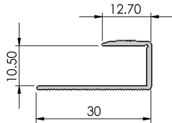
Section view
