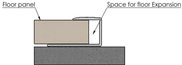
Typical installation detail
