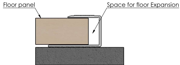
Typical installation detail
