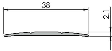
Section view
