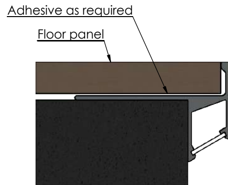
Typical installation detail
