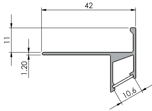
Section view
